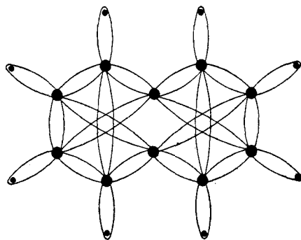
Fig. 6.—The structure of the naphthalene molecule.
